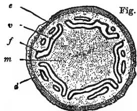
SECTION OF STEM OF TREE-FERN.† ( Cyathea. )
